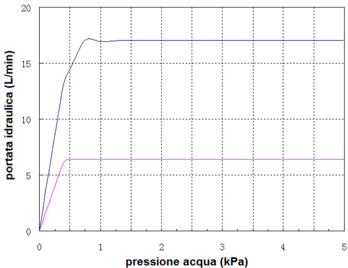
Infinity REU-1116FFU
