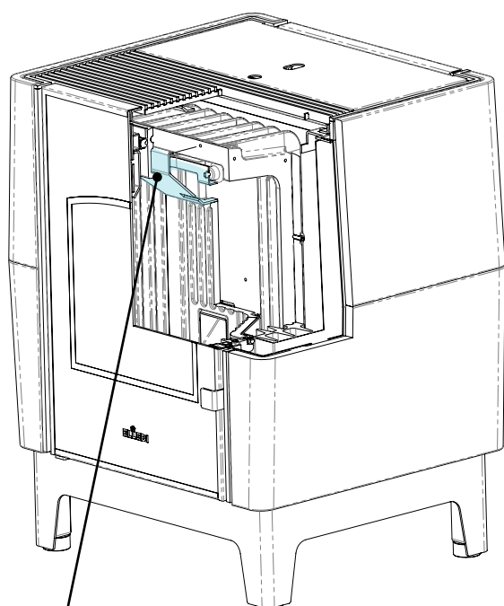
Flame trap in its seat
