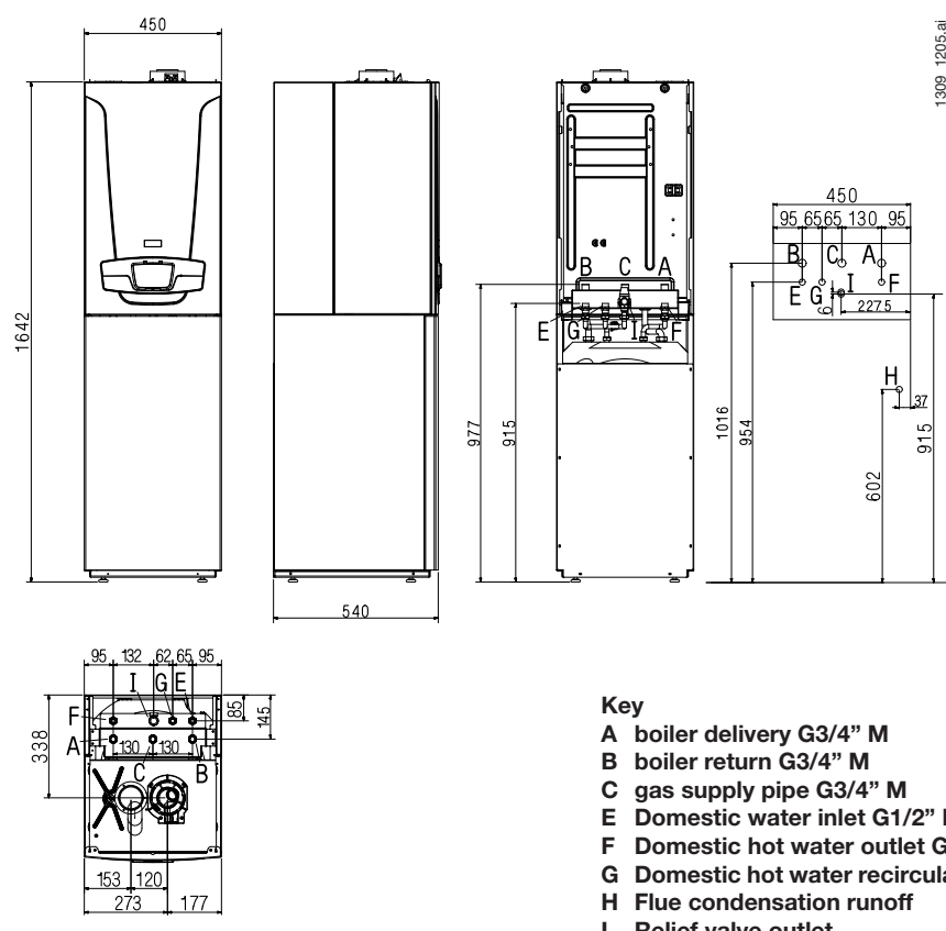
Appliance dimensions
