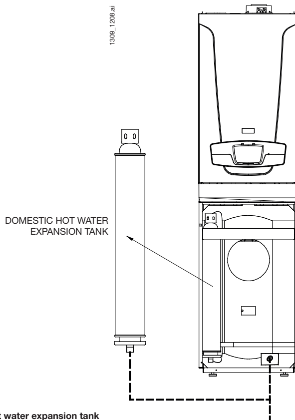
Figure 4: domestic hot water expansion tank
