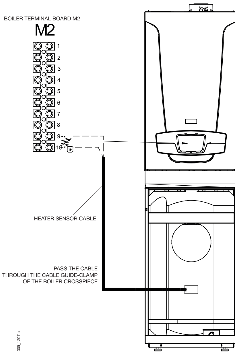
Figure 3: Domestic hot water priority sensor connection
