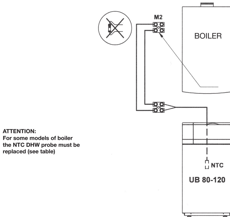
Figure 4: Connecting the NTC DHW priority probe
