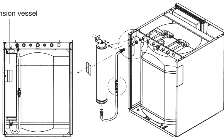
hydraulic connection
