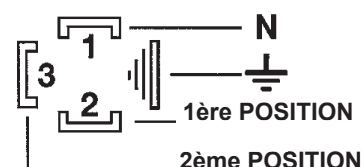
DETAIL BORNIER VANNE MB-ZRDLE
