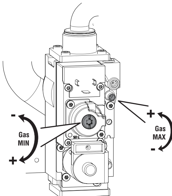
Valvola gas MULTIDEA EVO EXTRA 2.95 - 2.110 - 2.150
