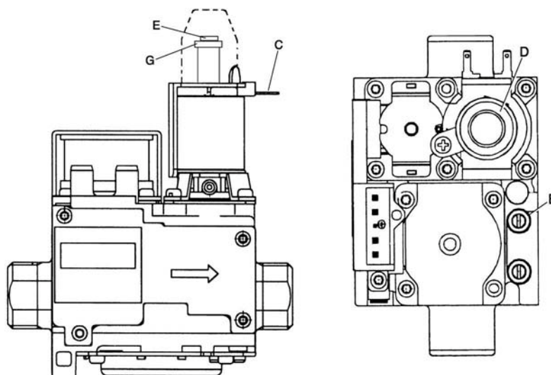
fig. 16 - Valvola gas
