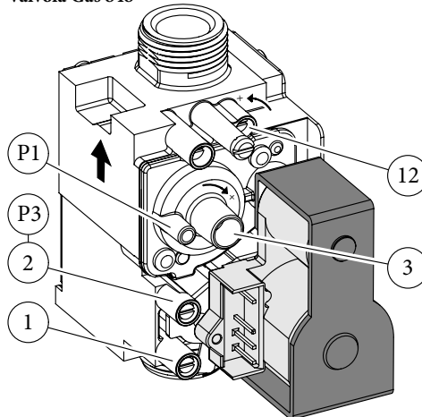
Valvola Gas 848
