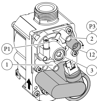
Valvola Gas 8205
