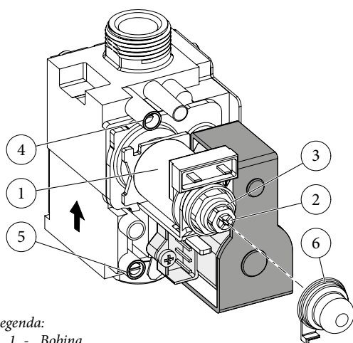
Valvola GAS SIT 845
