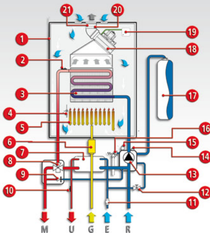
CIRCUITO IDRAULICO CLIZIA N 24/32 AS
