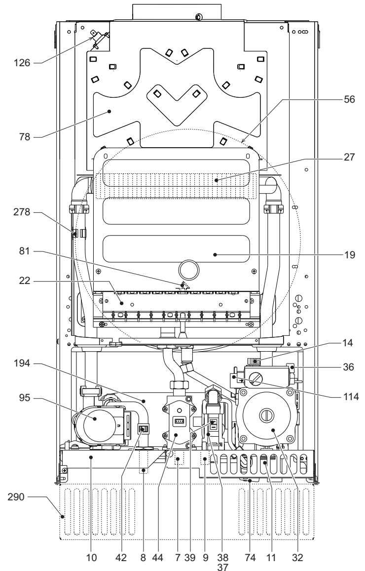
fig. 13 - General view CLIZIA D 24 A
