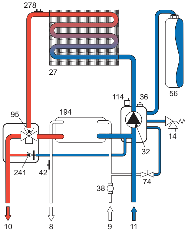
fig. 14 - Heating Circuit
