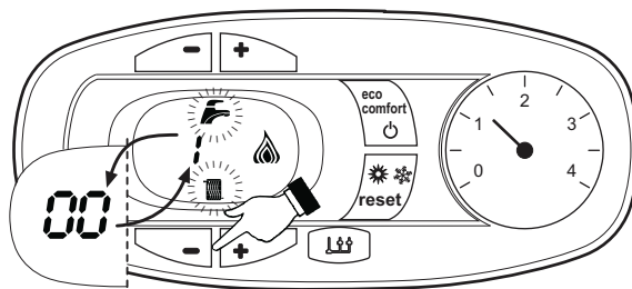
fig. 9 - TEST mode (heating power = 100%)
