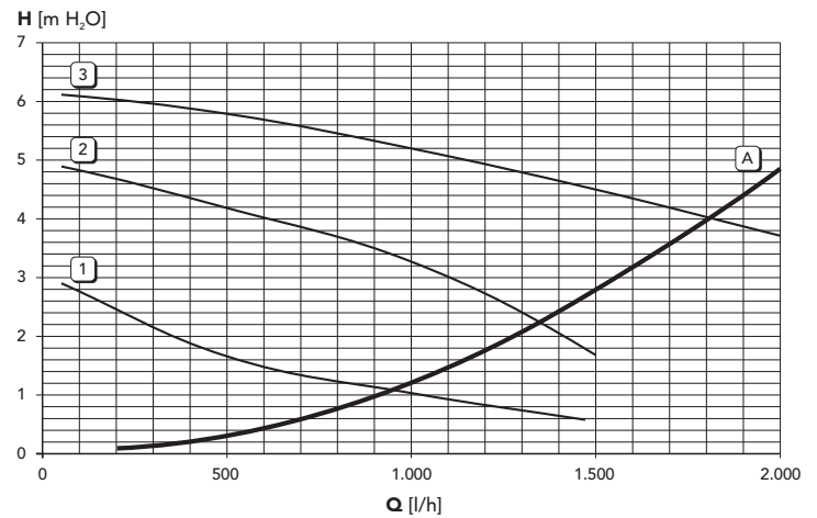
Circulating pump head / pressure losses CLIZIA D 32 A
