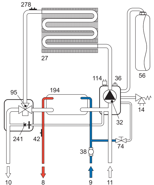
fig. 15 - Circuito de AS
