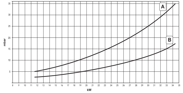
Circulating pump head / pressure losses CLIZIA D 32 A
