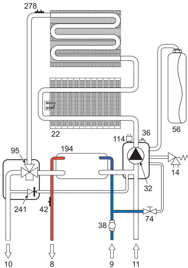
fig. 23 - DHW circuit
