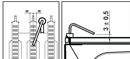
fig. 20 - Electrode positioning
