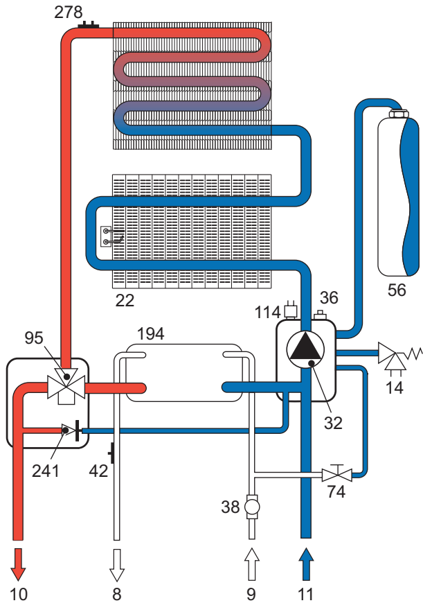
fig. 22 - Heating circuit
