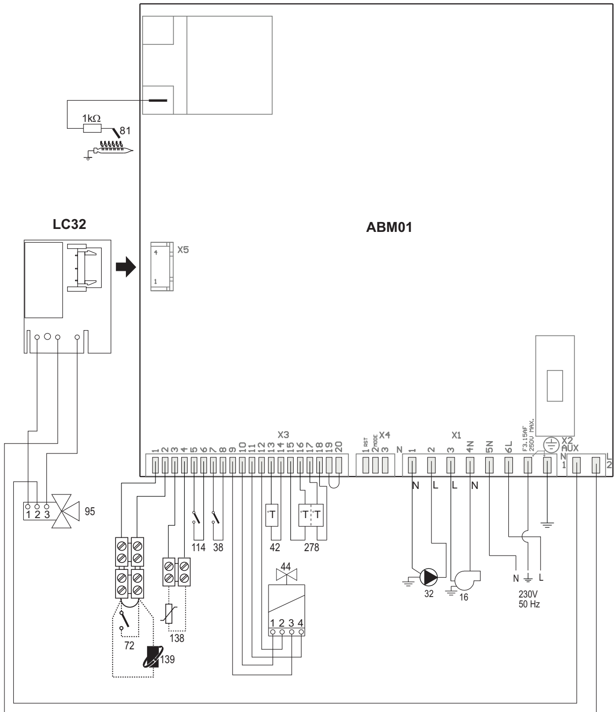
fig. 24 - Electrical circuit
