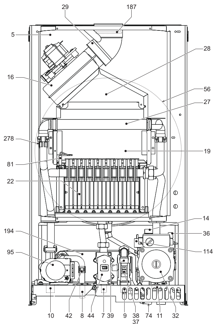
fig. 21 - General view
