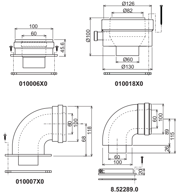
fig. 10 Starting accessories for coaxial ducts
