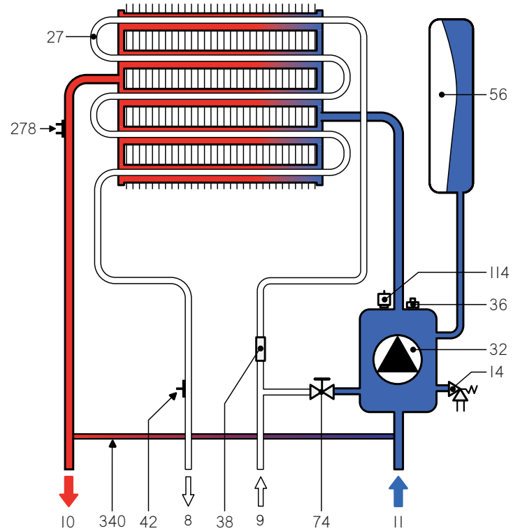
fig. 20 - Heating Circuit
