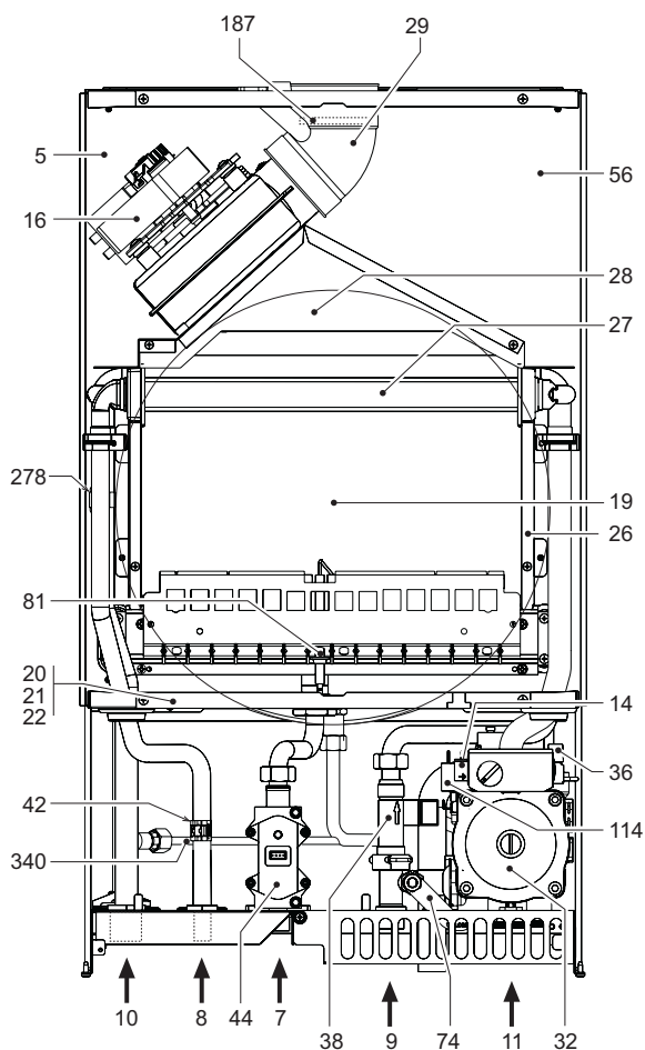
fig. 19 - Vista general CIPREA D 32 AS
