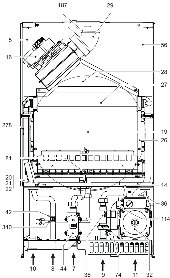
fig. 19 - General view CIPREA D 32 AS
