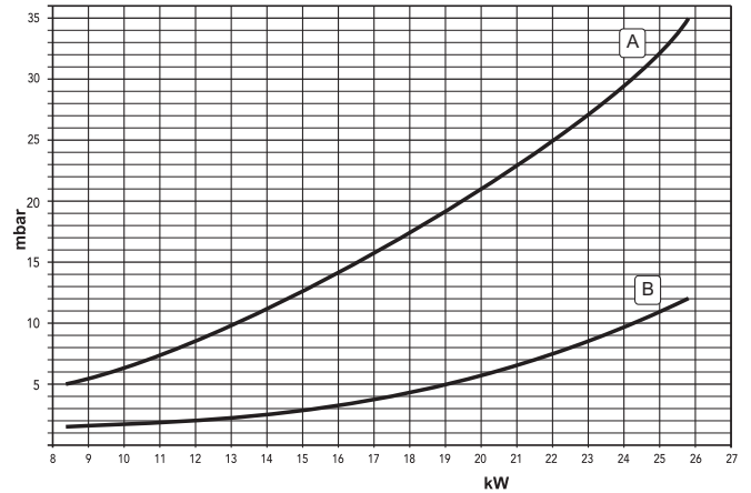
fig. 22 - Pressure - power diagram (CIPREA D 24 AS)
