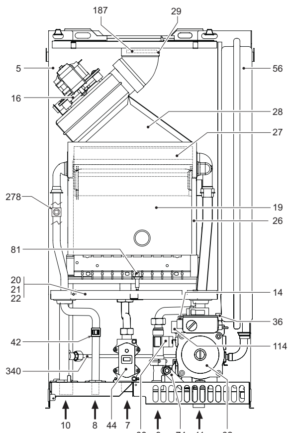
fig. 18 - Vista general CIPREA D 24 AS
