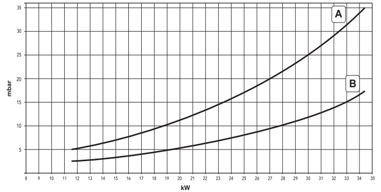
fig. 23 - Pressure - power diagram (CIPREA D 32 AS)
