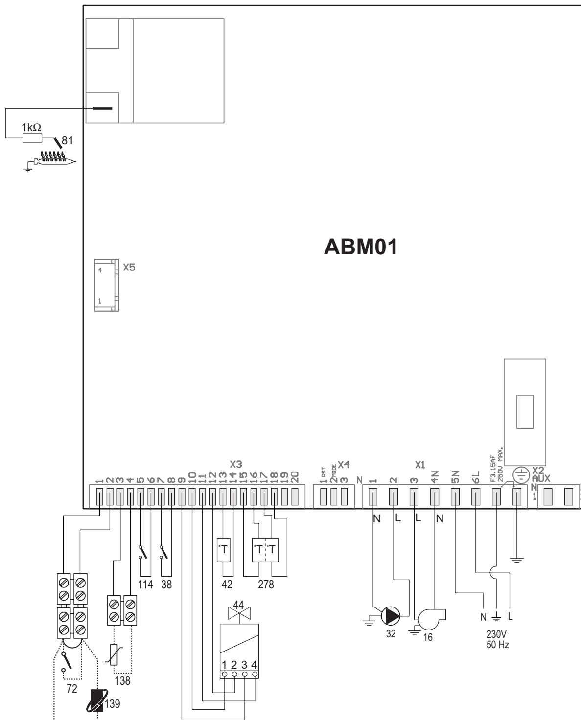
fig. 26 - Electrical circuit
