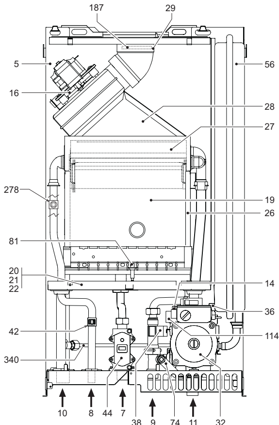
fig. 18 - General view CIPREA D 24 AS
