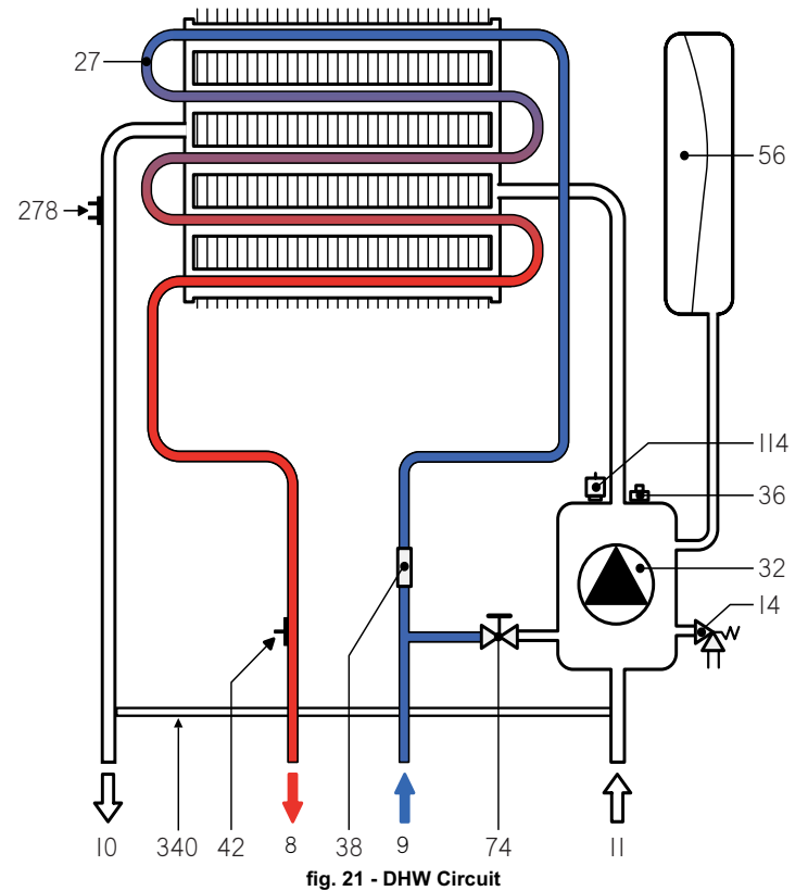
fig. 21 - DHW Circuit
