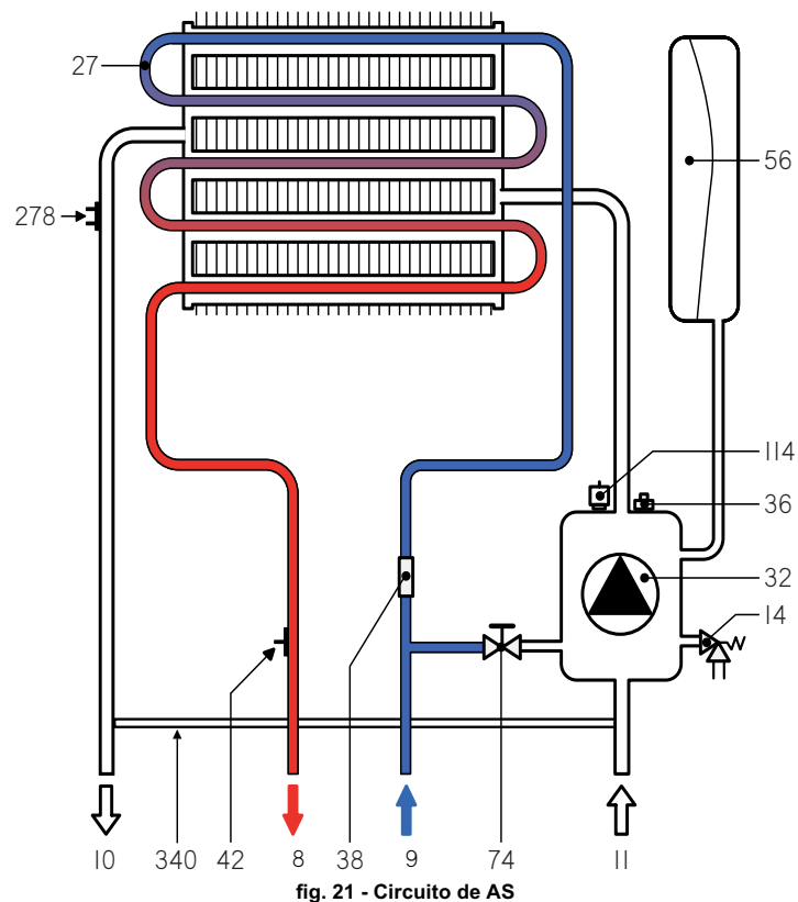
fig. 21 - Circuito de AS
