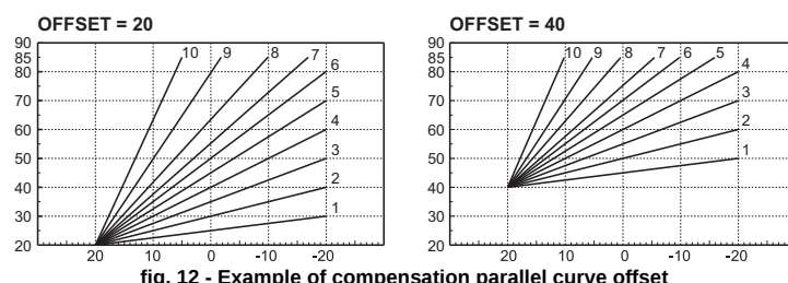
fig. 12 - Example of compensation parallel curve offset
