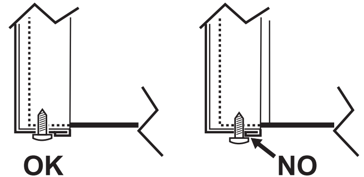
fig. 26 - Correct position of front panel
