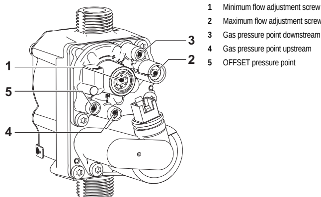
fig. 23 - Gas valve
