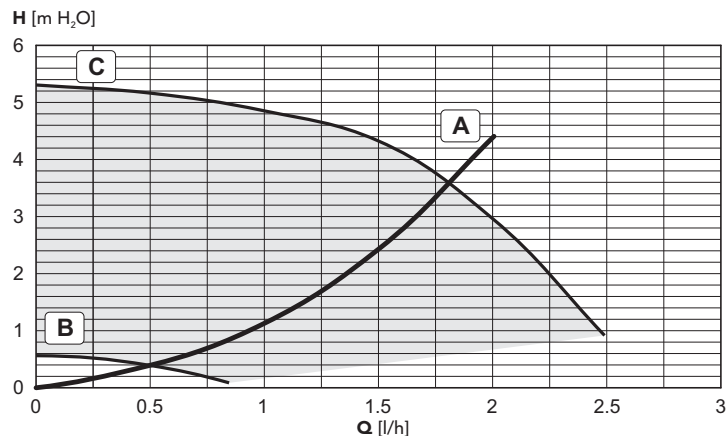
fig. 33 - Circulating pump head / pressure losses SILVER 24T
