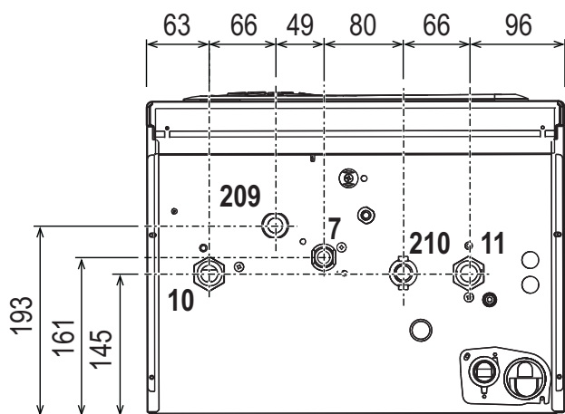
fig. 30 - Bottom view
