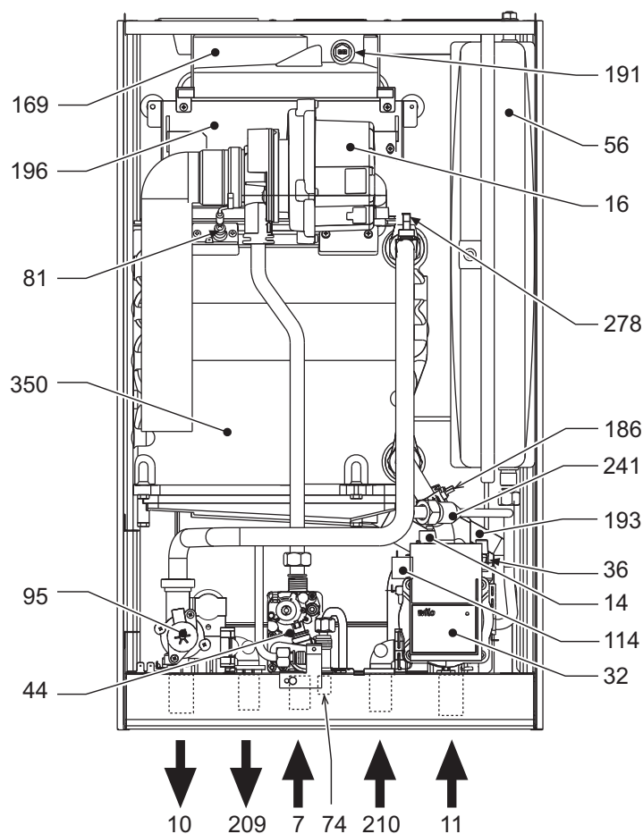
fig. 31 - General view
