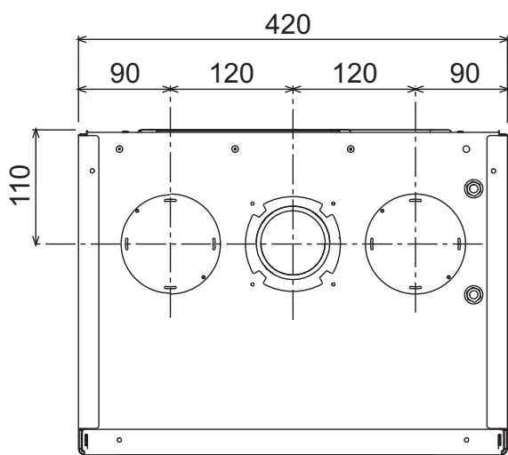
fig. 29 - Top view
