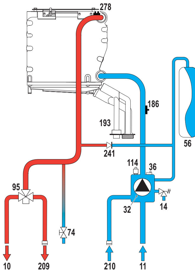
fig. 32 - Hydraulic circuit
