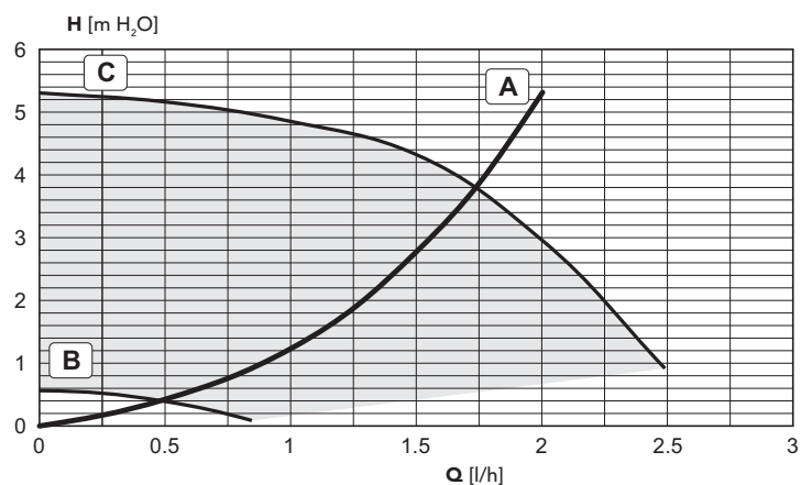
fig. 34 - Circulating pump head / pressure losses SILVER 34T
