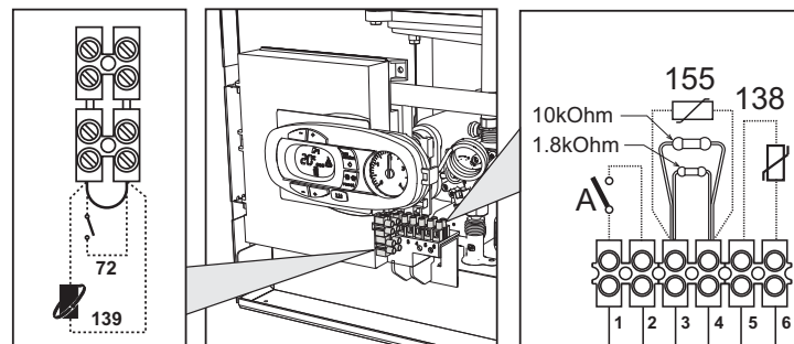
fig. 14 - Accessing the terminal block
