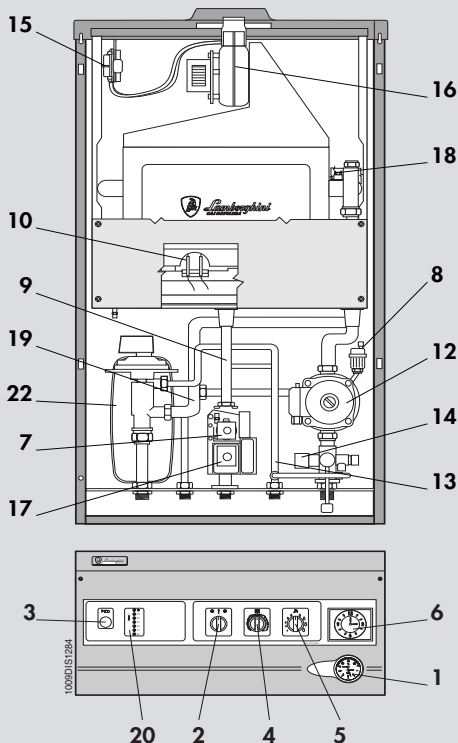
INOVA L20 MCS W TOP
