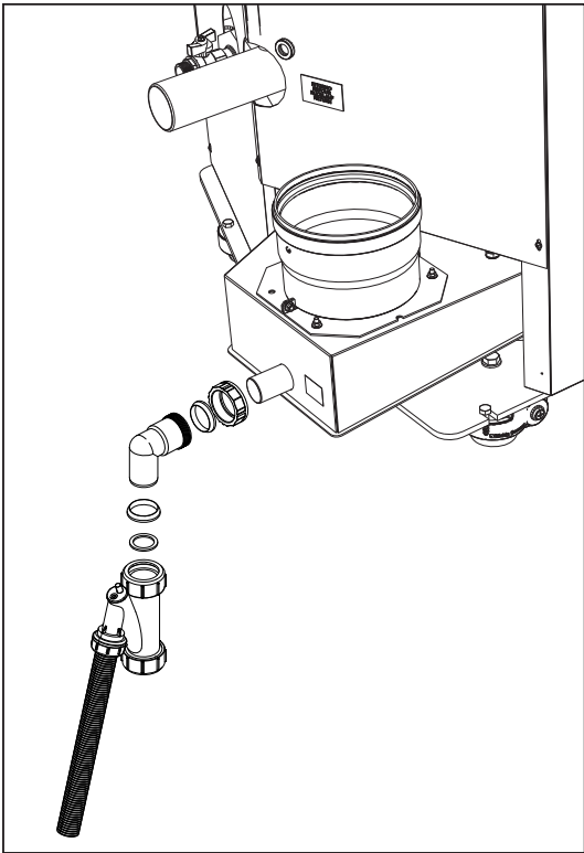
fig. 58- Condensate drain connection
