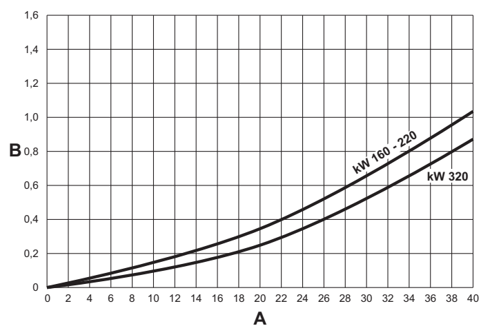
fig. 88 - Pressure loss diagram models 160, 220 and 320
