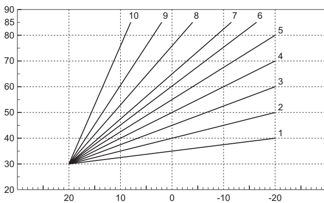
fig. 30- Compensation curves
