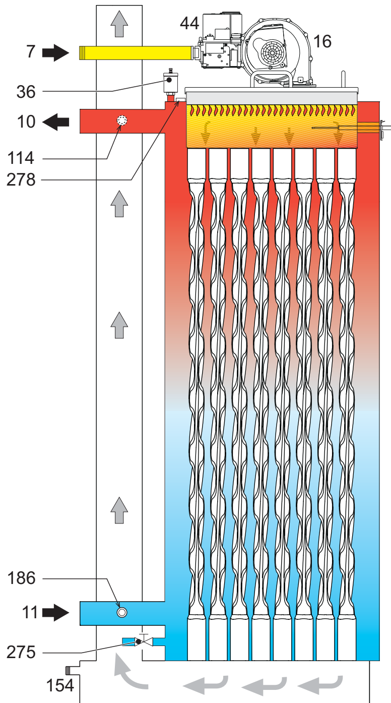
fig. 86- Hydraulic circuit
