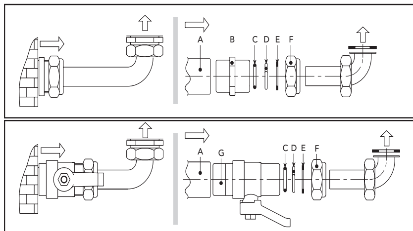
fig. 18 - Connection kits
