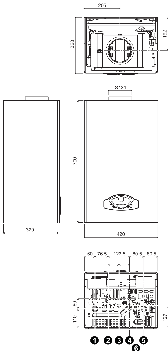
fig. 22 - Dimensions and connections
