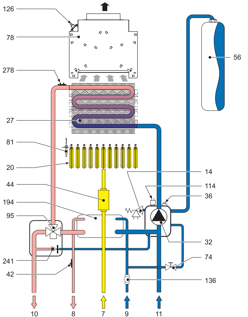
fig. 24 - Plumbing circuit
