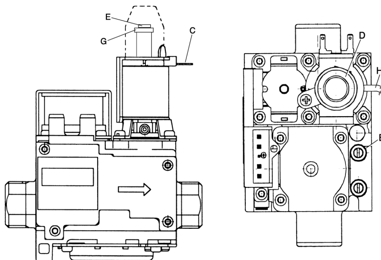
fig. 23 - Valvola gas
