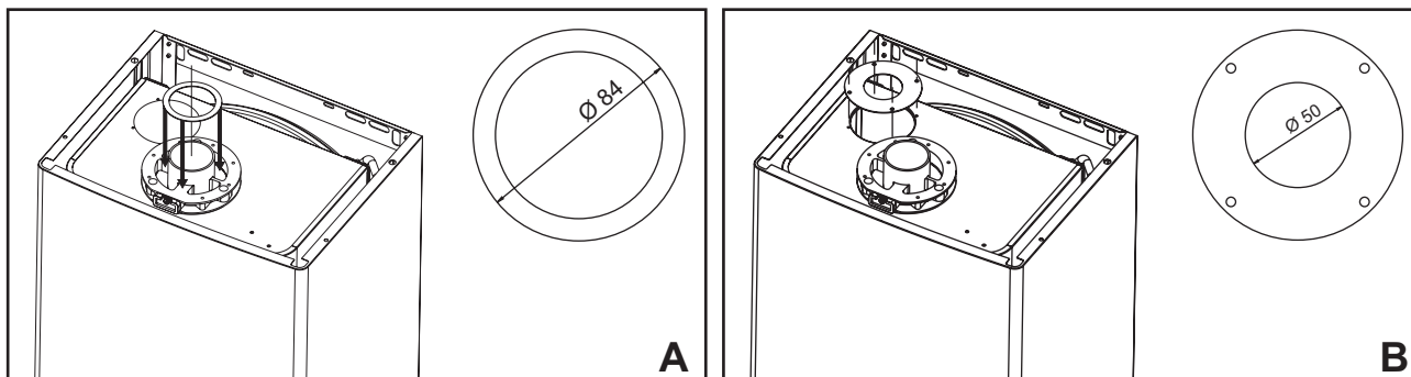
fig. 19 - Replacing the diaphragm
