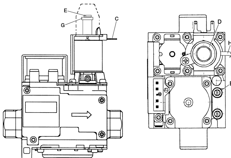
fig. 23 - Gas valve
