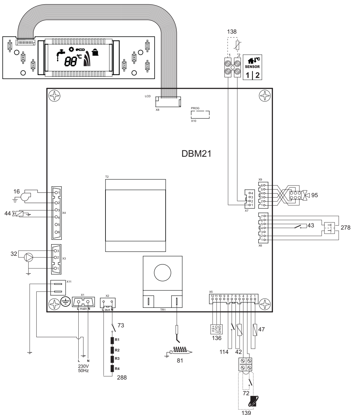
fig. 29 - Wiring diagram
