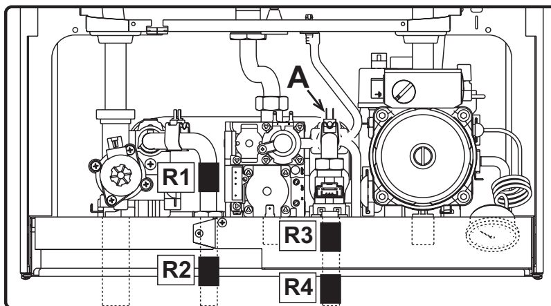
fig. 17 - Positioning of antifreeze thermostat and heaters
