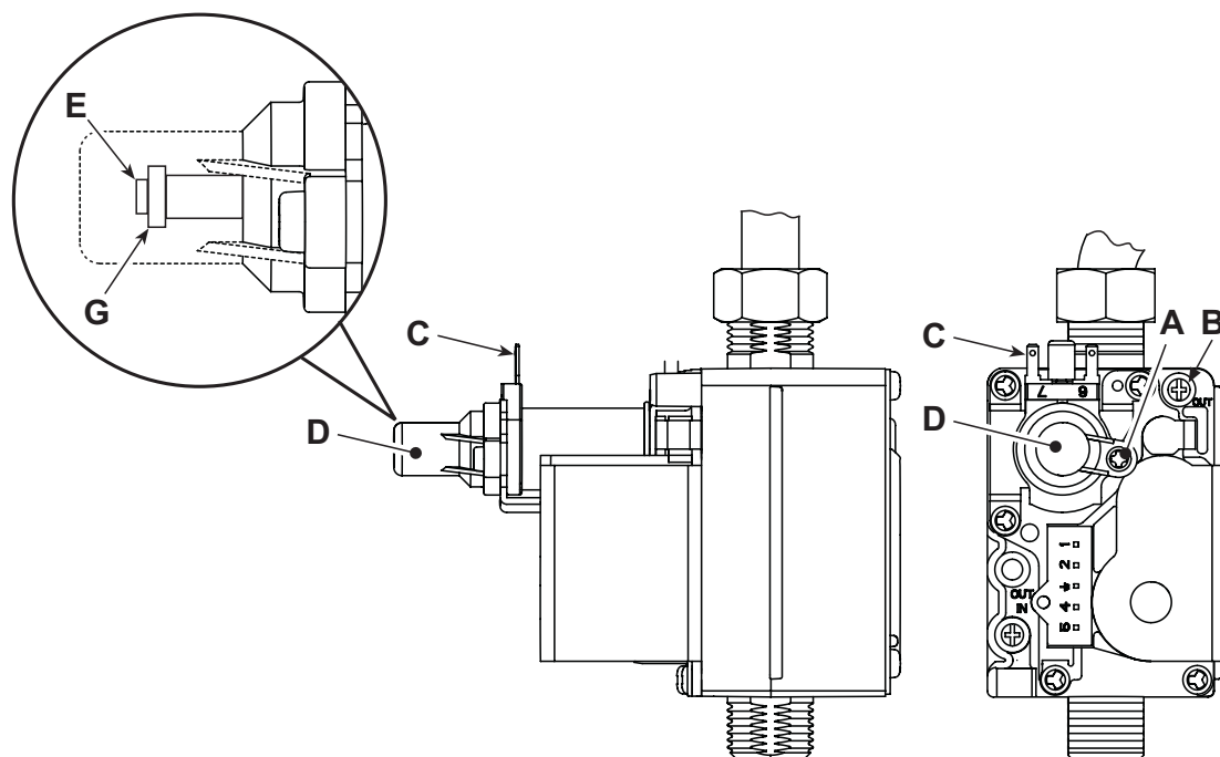
fig. 20 - Valvola gas
