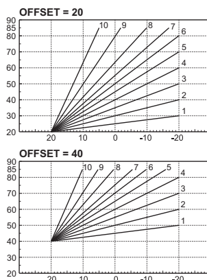
fig. 26- Example of compensation parallel curve offset
