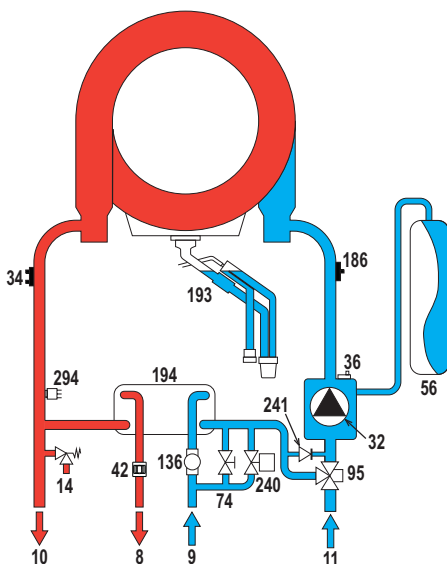
fig. 43- Hydraulic circuit
