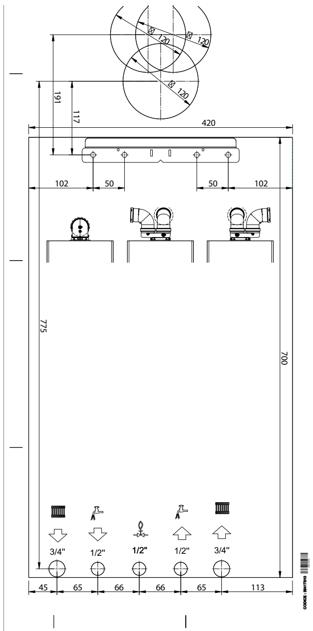
fig. 41- Paper template
