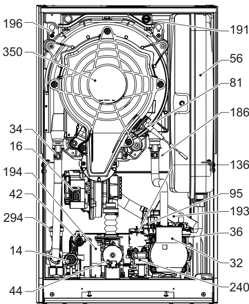
fig. 42- Vista general
