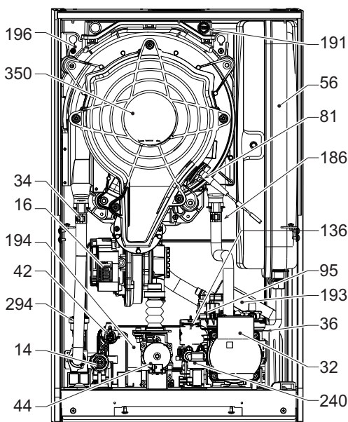
fig. 42- General view
