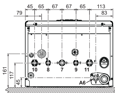
fig. 39- Bottom view
