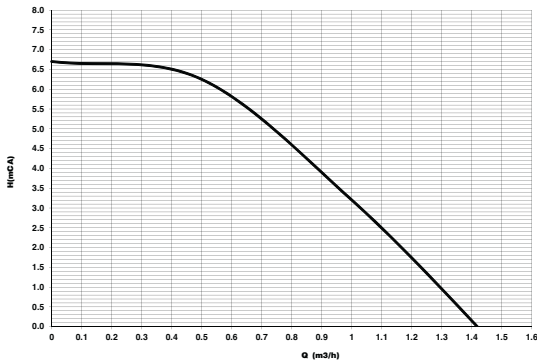
fig. 43- Residual head available for system
