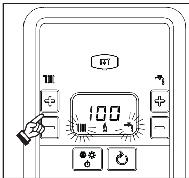
fig. 29- TEST mode (heating power = 100%)
