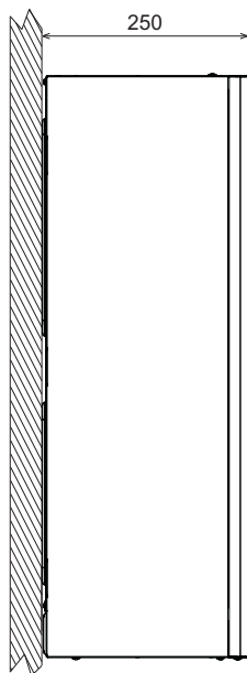
fig. 33- Side view
