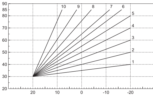
fig. 14- Compensation curves
