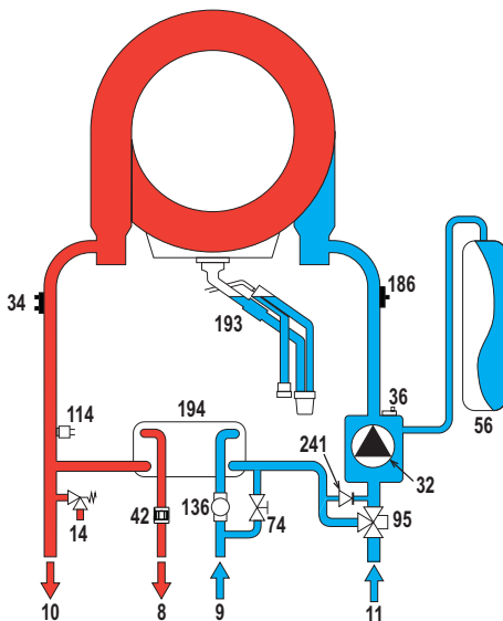
fig. 41- Hydraulic circuit
