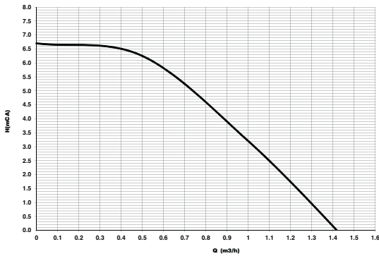
fig. 42- Residual head available for system
