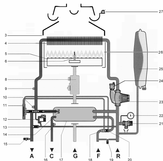
Figura 1-4 – Millennium E/26 E
