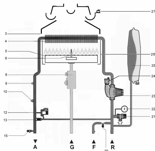
Figura 1-5 - Millennium RE/26 RE
