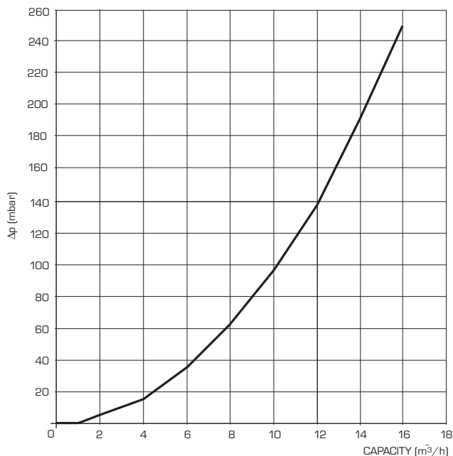
Hydraulic separator "DEWY EQUIPE 60-120-180-240 BOX/P60-P120 BOX"
