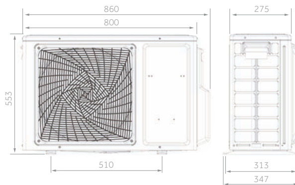
2U50S2SM1FA (2 attacchi)
