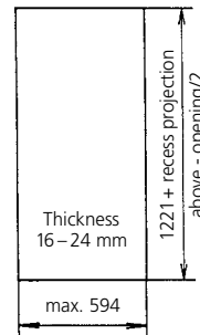
Door leaves EU
