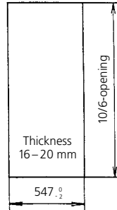
Door leaves CH
