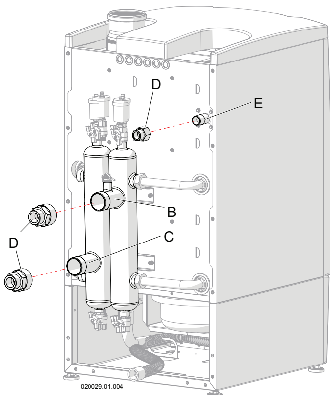
Figura 5-13 - Modelli 60T-70T-100T-115T-140T
