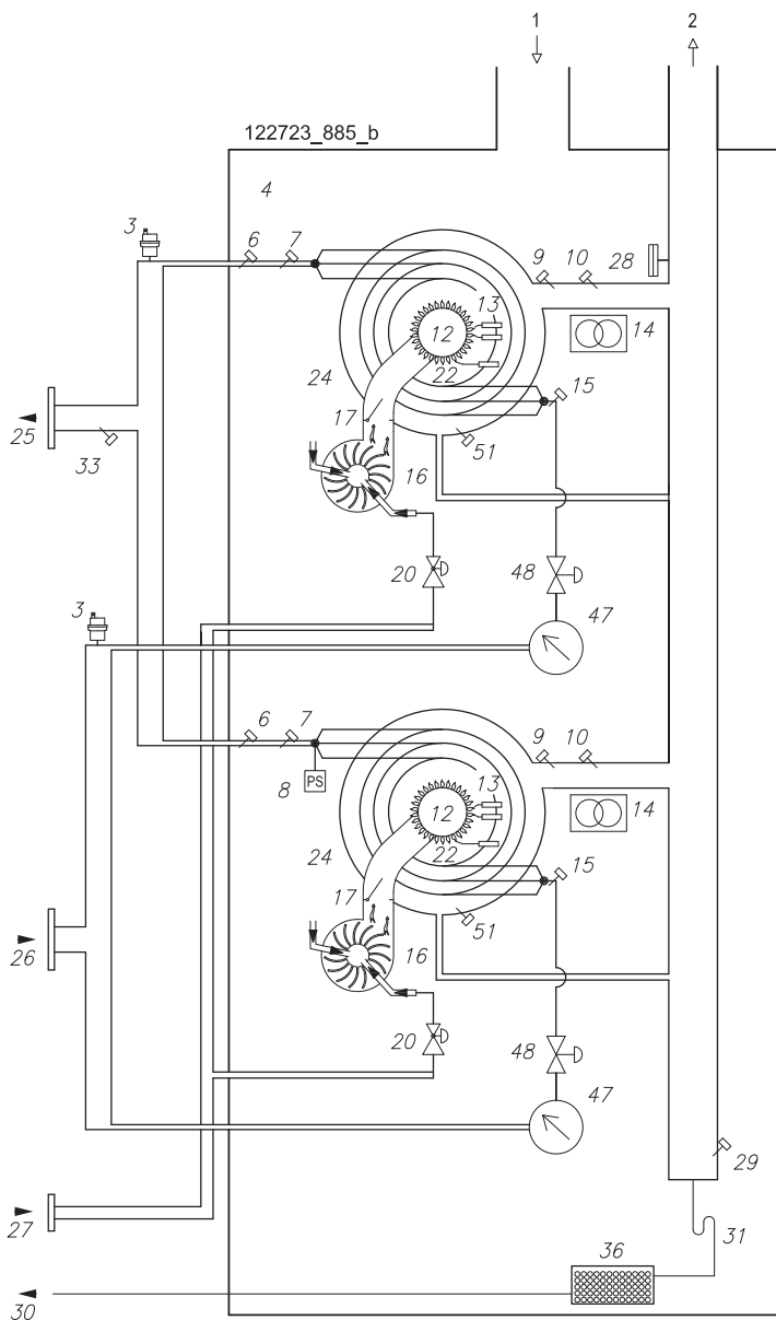
Figura 4-2 - Modelli 100T-115T-140T
