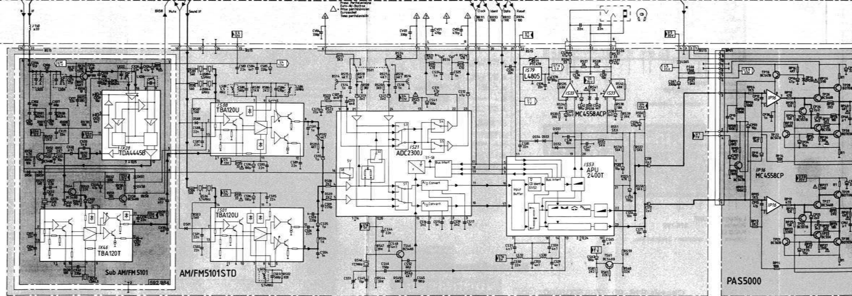
AM/FM-Tonmodul Modulo audio AM/FM 592.957 AM/FM sound module
