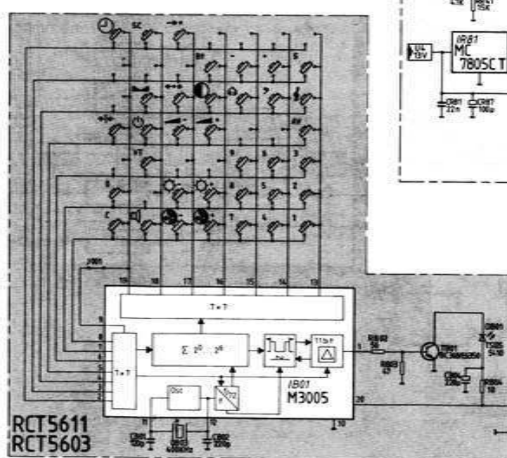
Infrarot-Fernbedienung Telecomando infrarossi Infra-red remote control Computer Control 6 583.559
